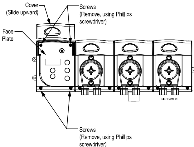
Figure 3. Opening Unit for Servicing
