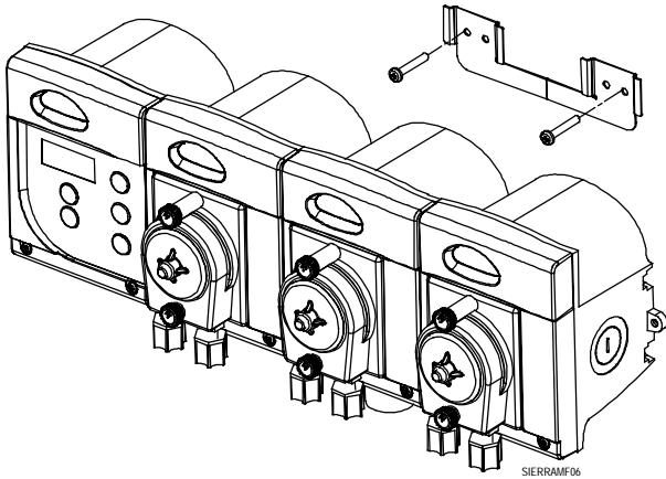
Figure 2. Sierra with Mounting Bracket
