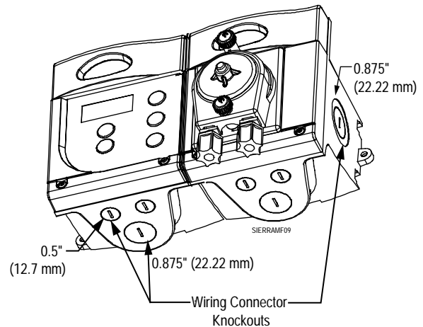
Figure 5. Bottom/Side Knockouts
