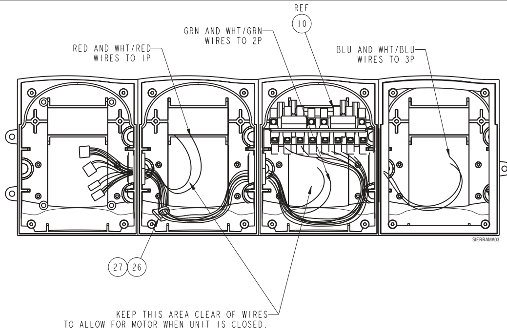
WIRE ROUTING
