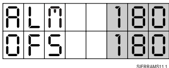
Screen 10. Detergent Alarm Timeout/Over Feed Stop Timeout Programming
