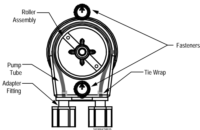
Figure 8. SnapHead Pump
