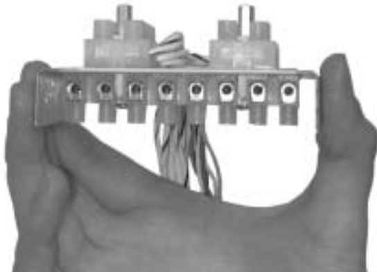
Figure 6. Sierra Wiring/Removable Terminal Blocks
